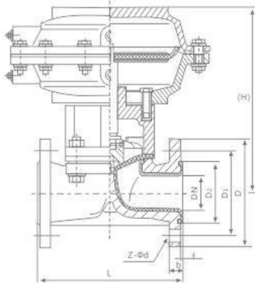
Eg641 F 46 型气动隔膜阀(堰式) EG641- F 46 Pneumatic diaphragm valve (weir type) 法兰连接隔膜阀 (英标) Flange connection diaphragm valve (British sign) ※设计与制造符合BS英国国家标准 Design and manufacture conform to BS Britain national standards ※公称压力PN0.6~1.6MPa Nominal pressure PN0.6~1.6MPa ※基本结构形式：堰式、直流式 Basic structure form: Weir, DC style ※公称通径DN20~200mm Nominal size Dn20~200mm
