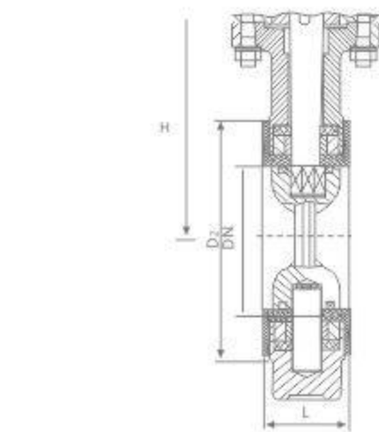
DA371F46型对夹式蜗轮传动蝶阀 (中线) DA371F46 Worm drive type wafer type butterfly valve (middle)
