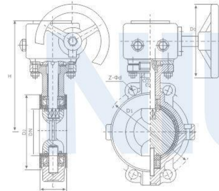
DA371F46型对夹式蜗轮传动蝶阀 (中线) DA371F46 Wafer type butterfly valve worm gear transmission (middle)
