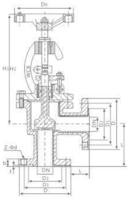
J44 F 46 型法兰连接手动截止阀 (角式) Flange connection manual cut-off valve (angle type)
